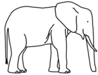
elephant
